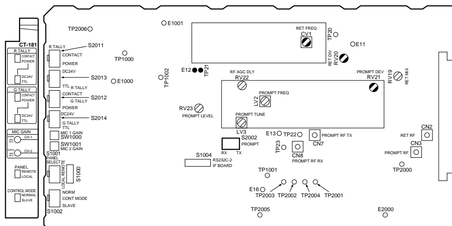
CT-181 Board (A SIDE)
