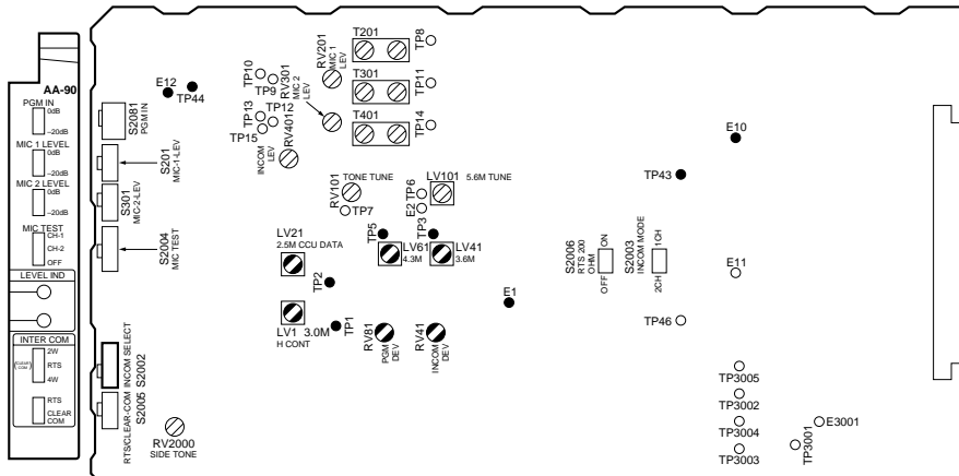
AA-90 Board (A SIDE)
