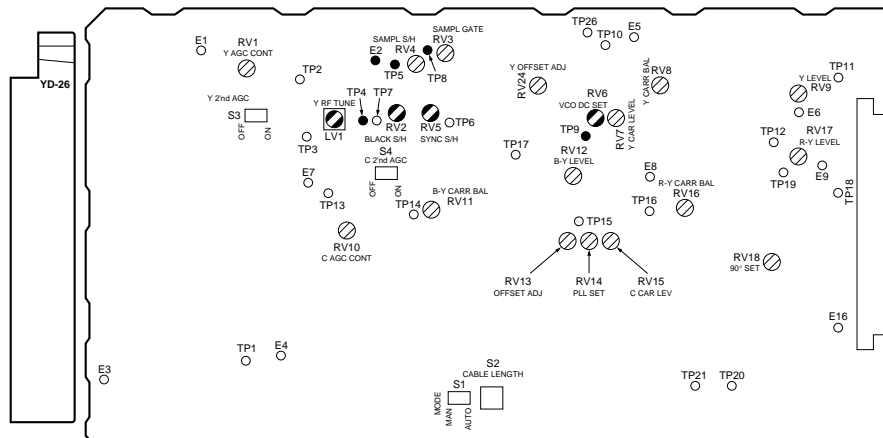
YD-26 Board (A SIDE)
