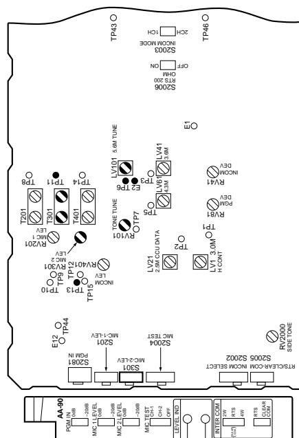
AA-90 Board (A SIDE)
