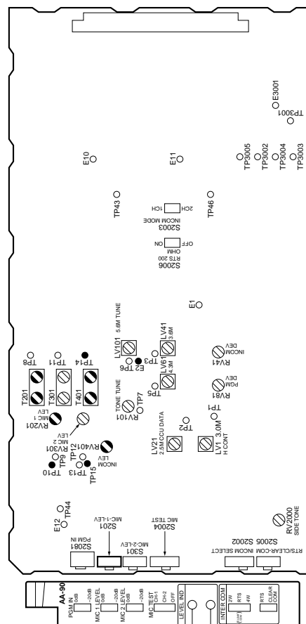
AA-90 Board (A SIDE)
