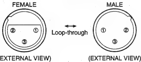
(EXTERNAL VIEW)
