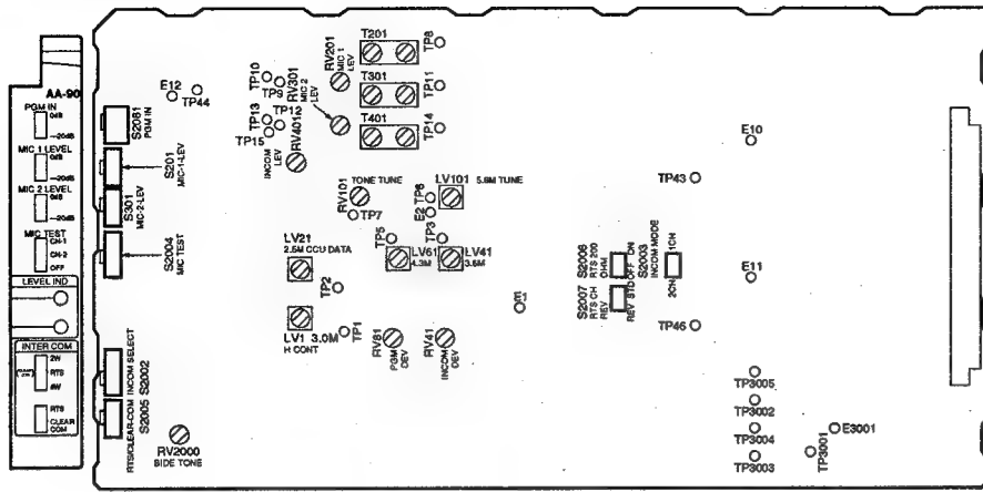
AA-90 Board (A SIDE)
