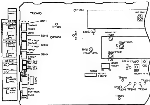
CT-181 Board (A SIDE)
