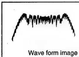
Wave form image CENT FREQ : 3.6 MHz FREQ SPAN : 20 MHz
