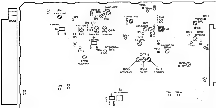
YD-26 Board (A SIDE)
