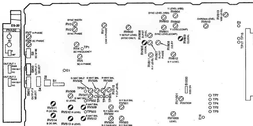
ES-20 Board (A SIDE)
